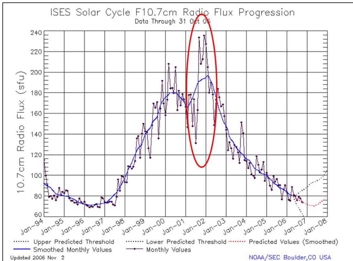
Figure 2: NOAA SEC solar flux (10.7cm) during cycle 23. Note the second solar max with extremely high flux from September 2001 to April 2002.
