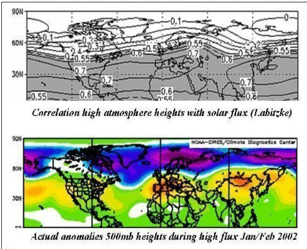
Figure 3: Labitzke correlated stratospheric heights with solar flux and actual height anomalies in the mid-troposphere during the high flux mode of the second solar max in early 2002.
